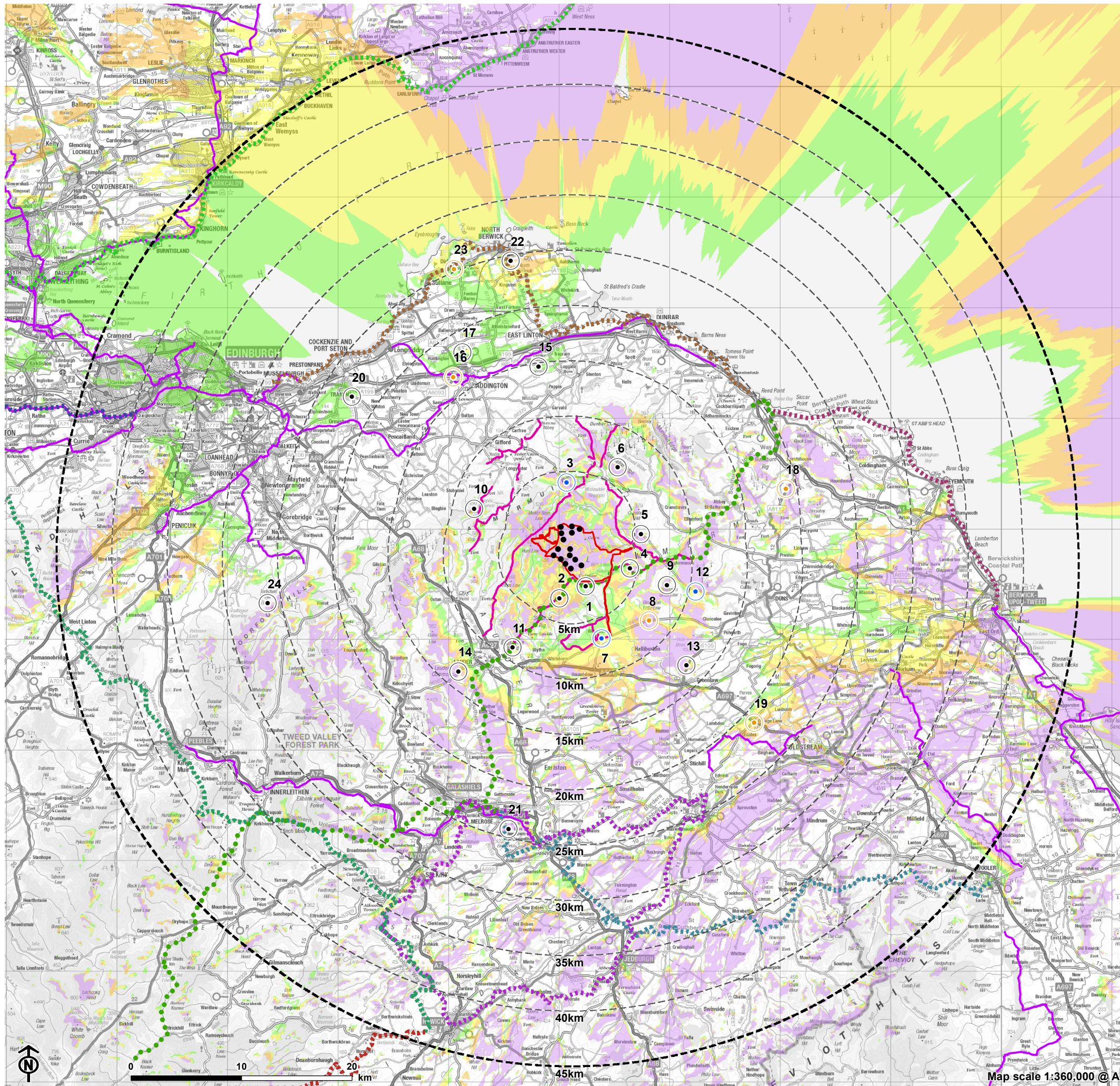
Figure 4.1.3a: Turbine Hub Height (130m) Zone of Theoretical Visibility (ZTV) and Viewpoint Locations
