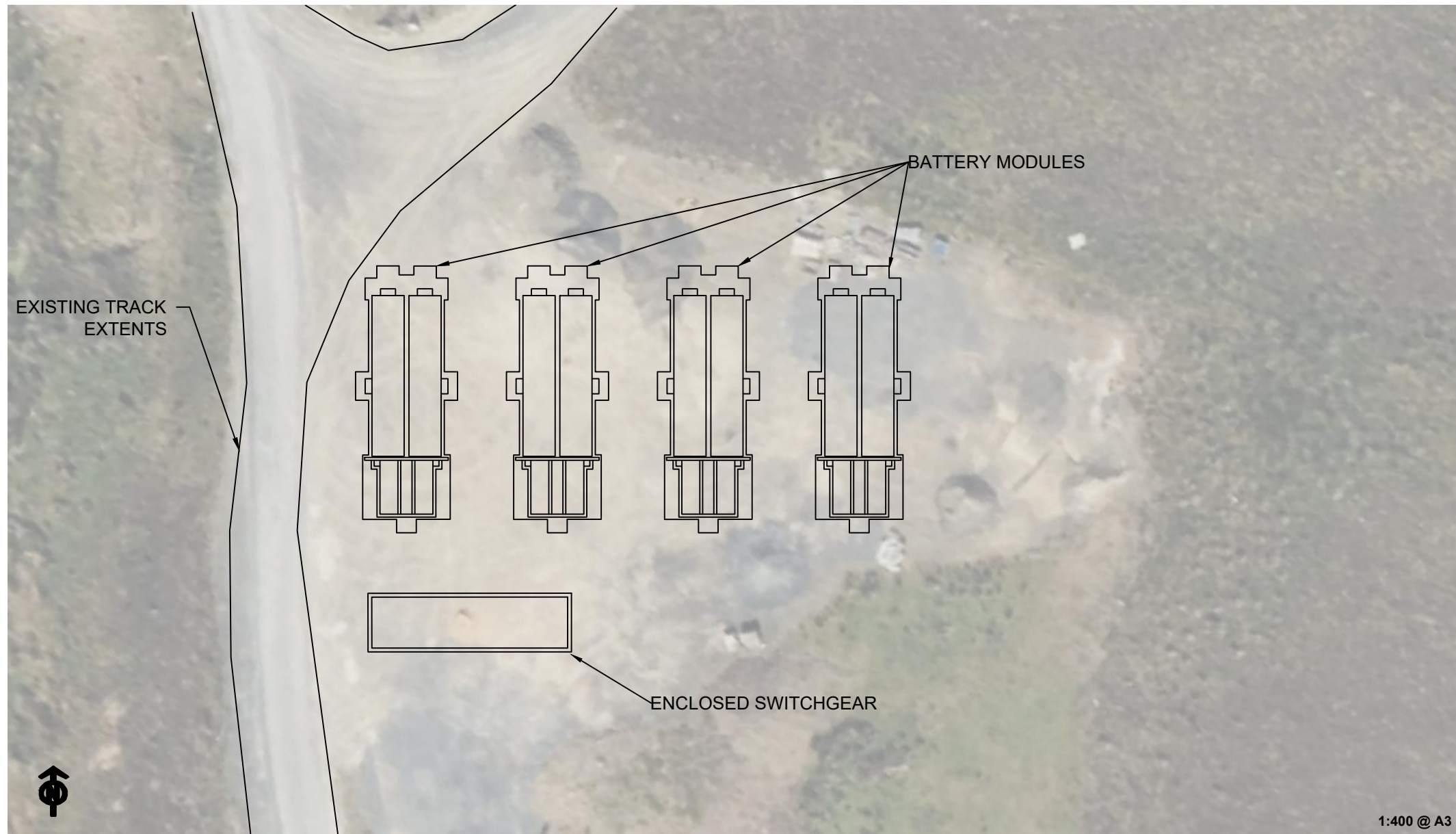
Figure 3.7: Indicative Battery Storage Facility
