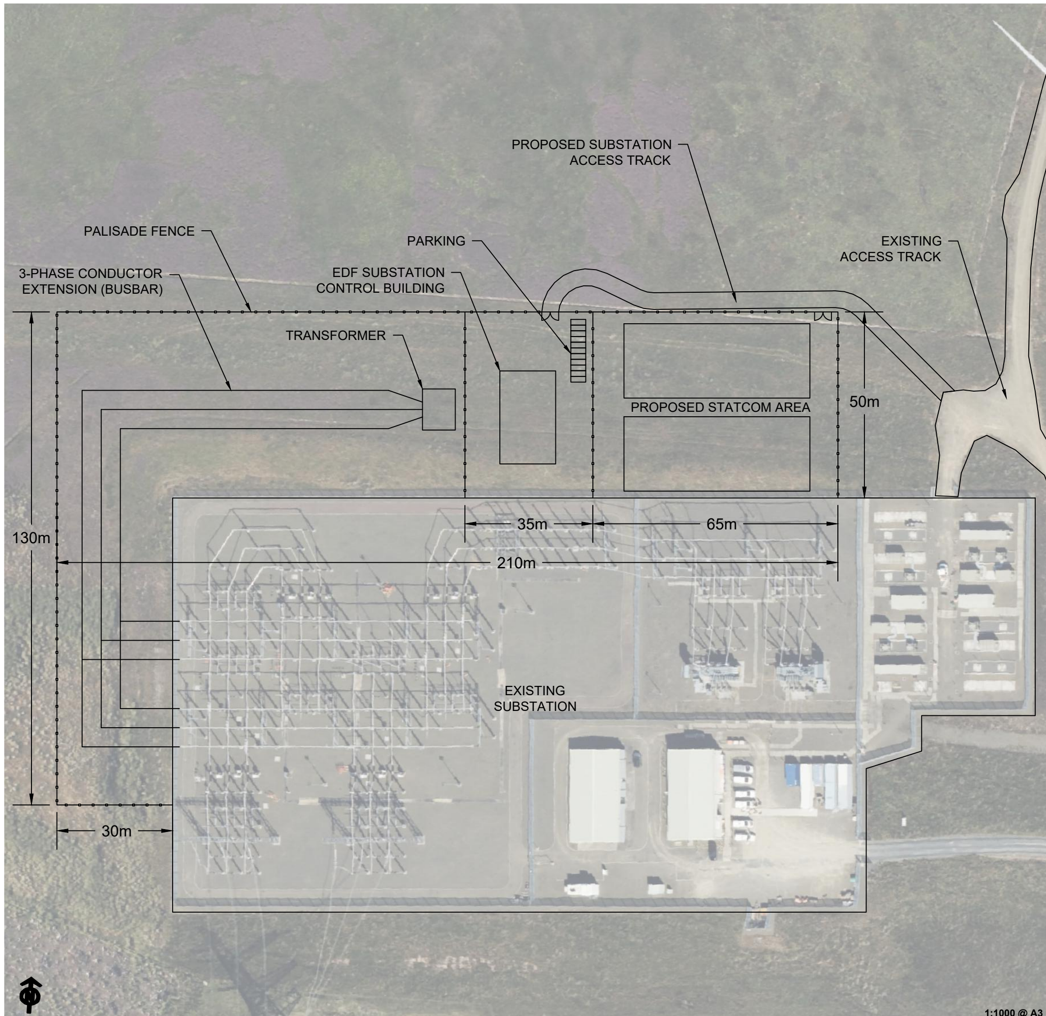
Figure 3.6: Proposed Substation Expansion
