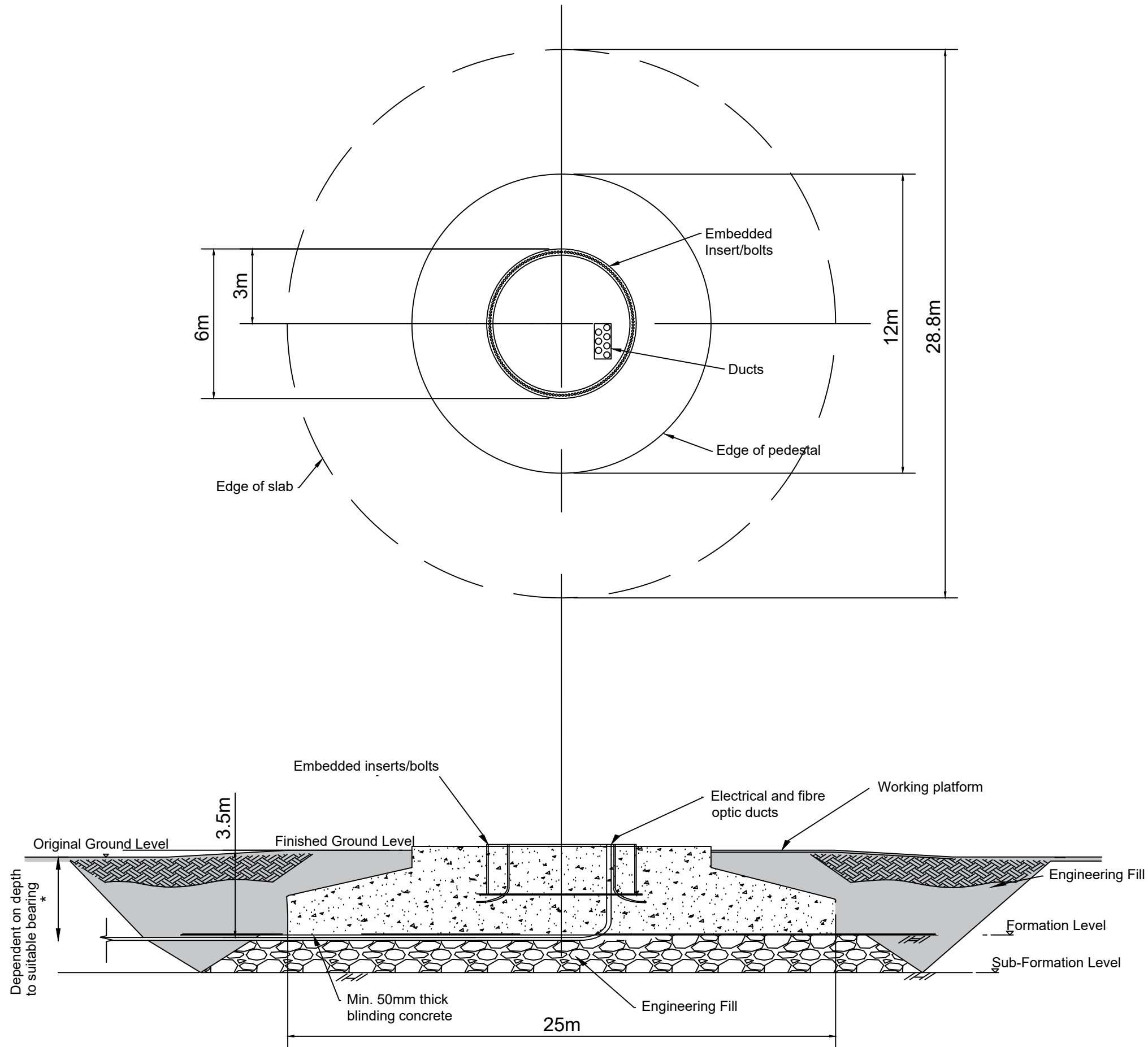
Figure 3.3: Typical Turbine Foundation
