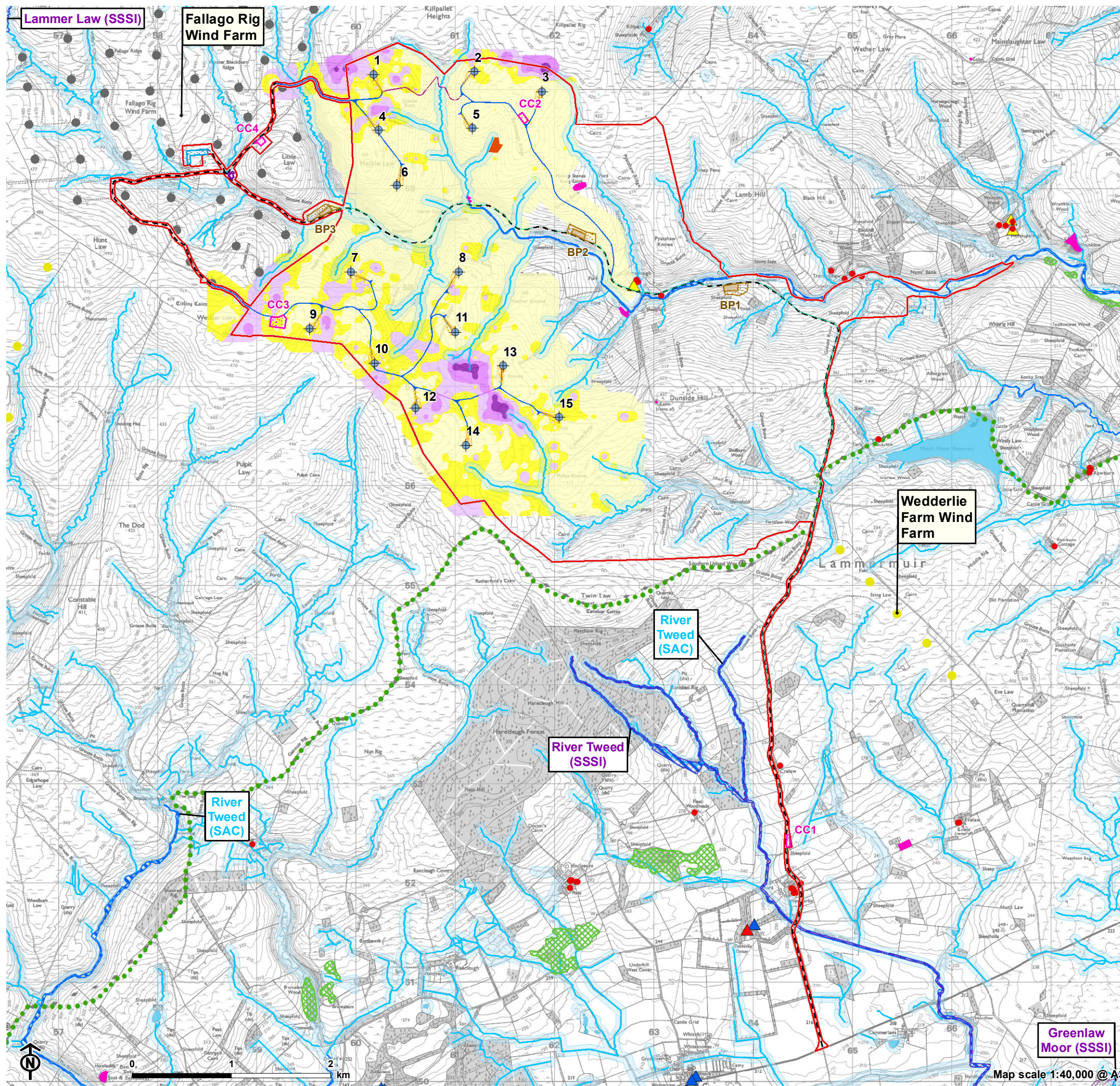
Figure 2.4: Site Constraints
